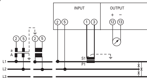
Three-phase line 3 wire, balanced load
