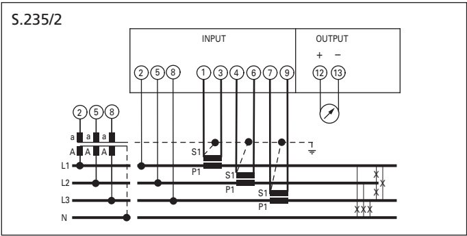
Three-phase line 4 wire, unbalanced load
