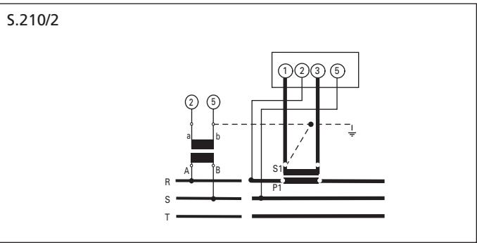
Three-phase line 3 wire, balanced load
