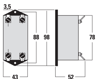
Rectifier accessory for a.c. ammeters AQ48M/rad
