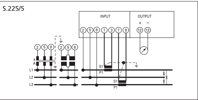
Three-phase line 3 wire, unbalanced load ARON
