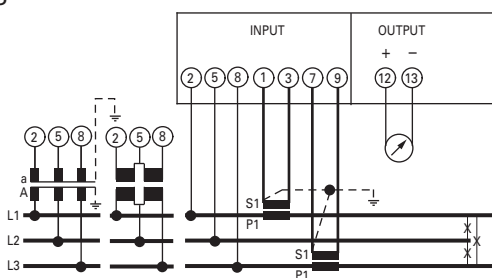
Three-phase line 3 wire, unbalanced load ARON
