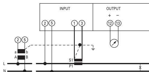
Single-phase line
