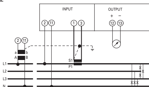
Three-phase line 4 wire, balanced load
