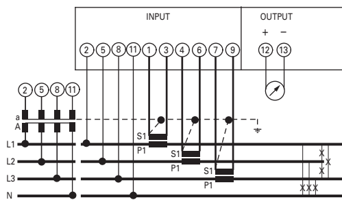
Three-phase line 4 wire, unbalanced load
