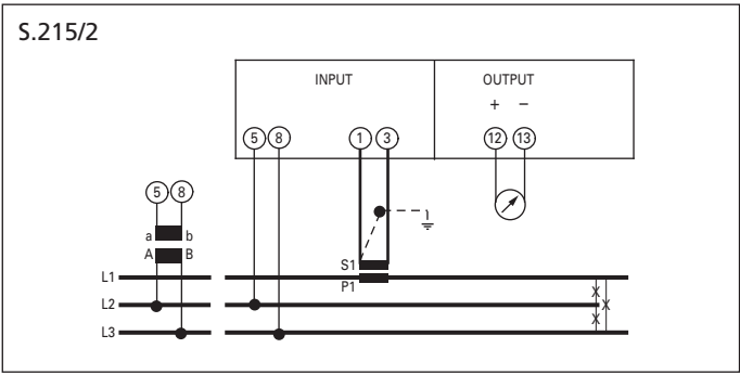
Three-phase line 3 / 4 wire, balanced load
