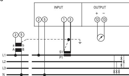
Single or Three-phase line 4 wire, balanced load
