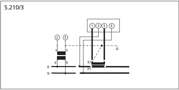
Single or Three-phase line 4 wire, balanced load
